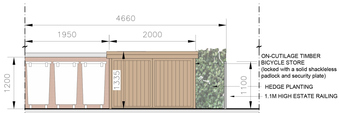
SIDE ELEVATION Scale 1:50
