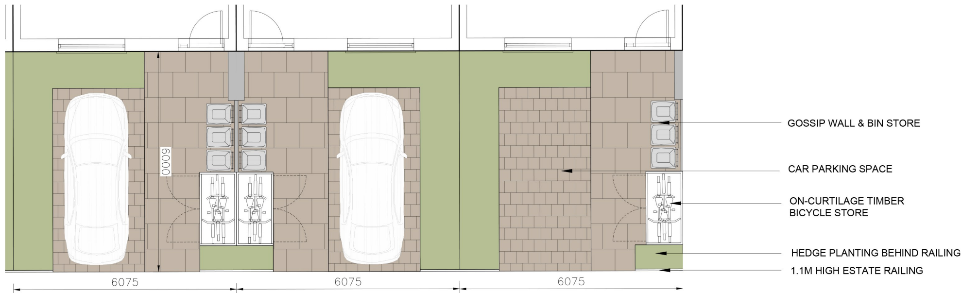
TYPICAL MID-TERRACE CURTILAGE PLAN Scale 1:100 (Refer to Landscape Architect's Drawings for boundary specifications and details)
